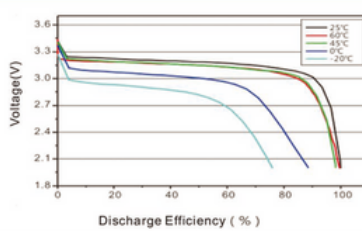
Temperature Characteristics
