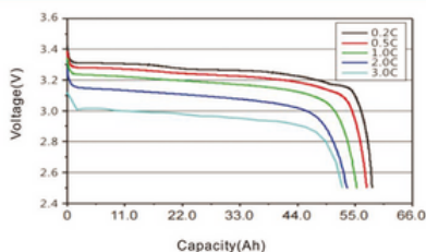
Discharge rate curves
