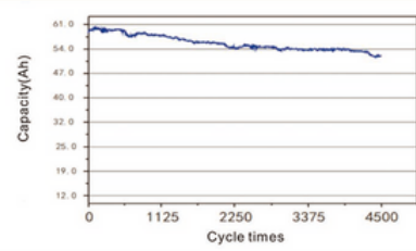
Cycle curves of 4500 times
